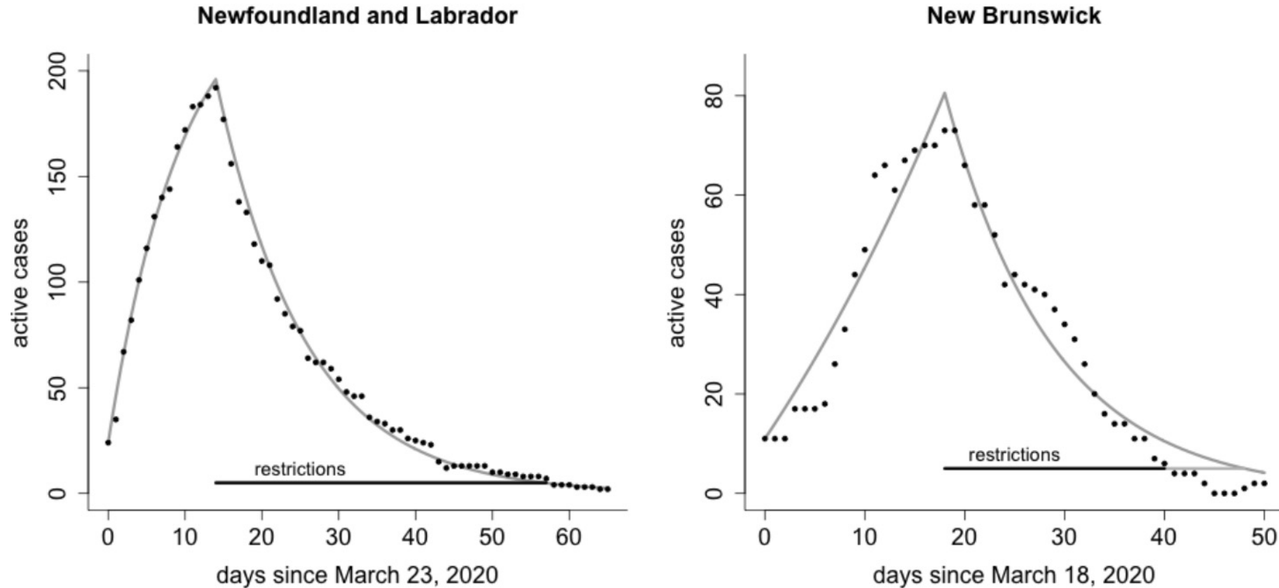
Fig. 1 The linear SIR model fitted to data describing the active number of COVID-19 cases in Newfoundland and Labrador and New Brunswick from March-May, 2020. Equation 1a,
